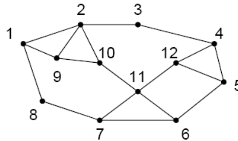
(a) undirected graph
