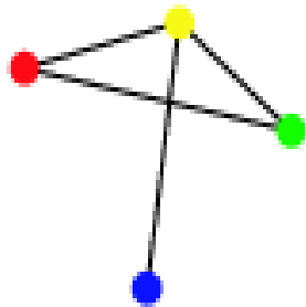
vertex-colored graph
