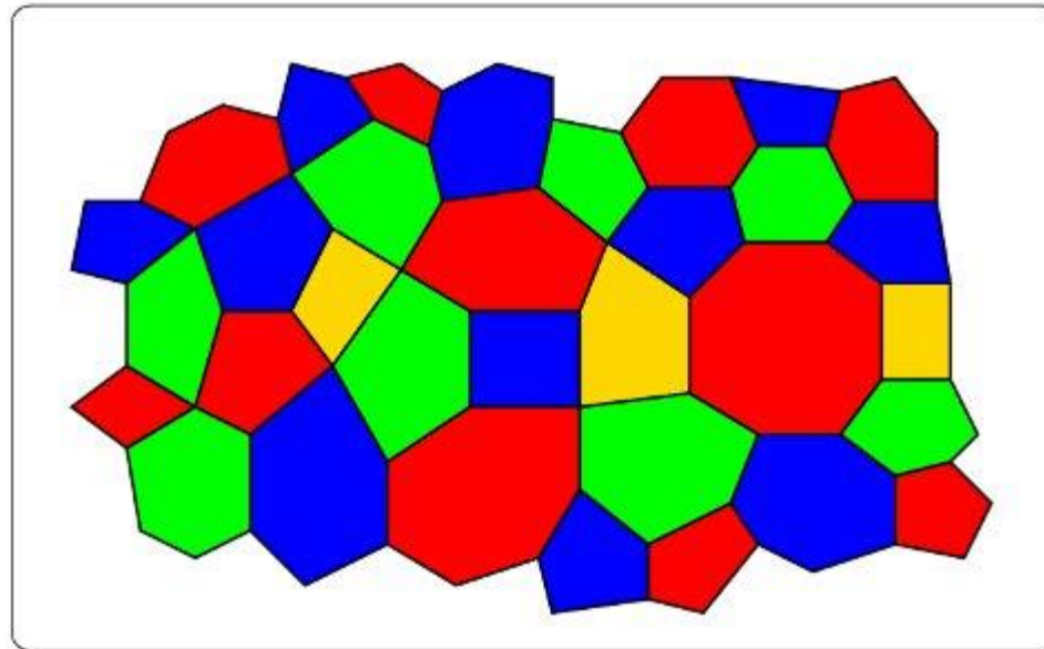
4-Colored Map
