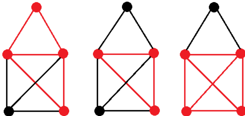
not a clique
