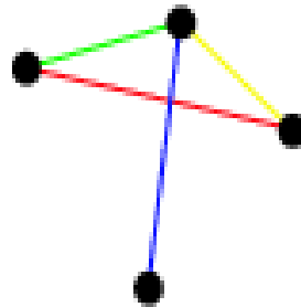
edge-colored graph
