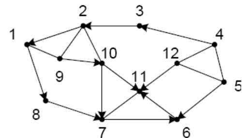
(b) directed graph
